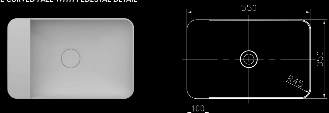
THE CARRE BEAUTIFUL CURVED FALL WITH PEDESTAL DETAIL
