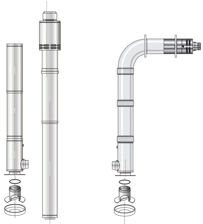
3m Top Flue Set DBV26FST (26kW) DBV36FST (36 & 46kW)
