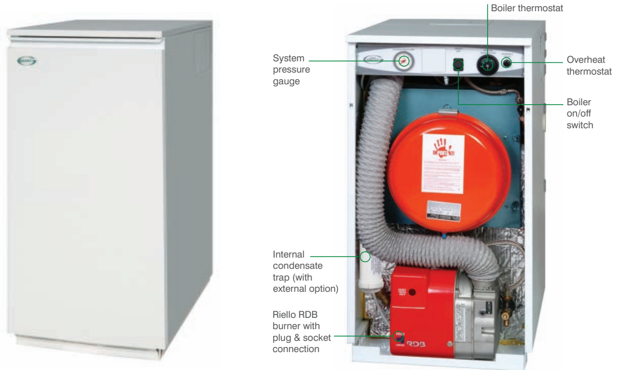
Model shown: DBV26 (front view)
