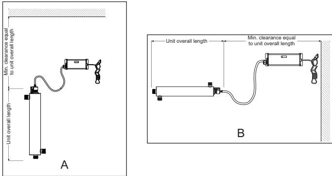
Figure 3 Disinfection Installation - Vertical and Horizontal
