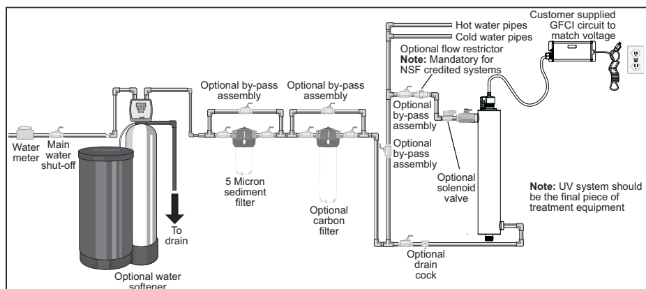
Figure 2 Disinfection System
