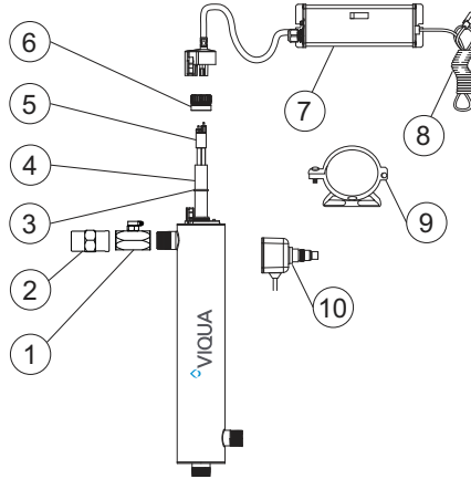
Figure 1 System Components
