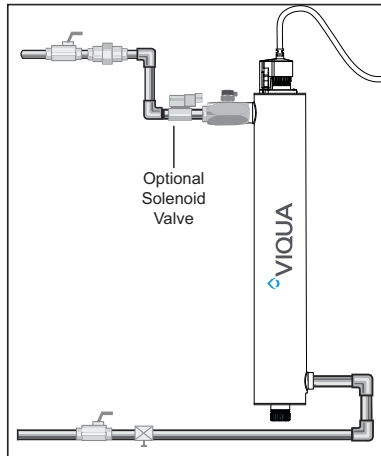
Figure 1 Solenoid Installation
