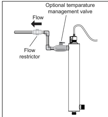
Figure 4 Flow Restrictor
