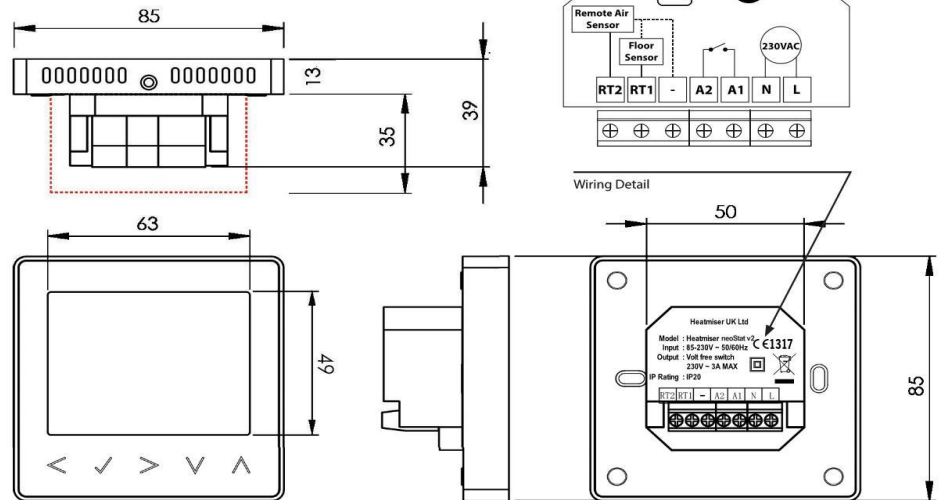
Product Dimensions (mm) & Wiring Specification
