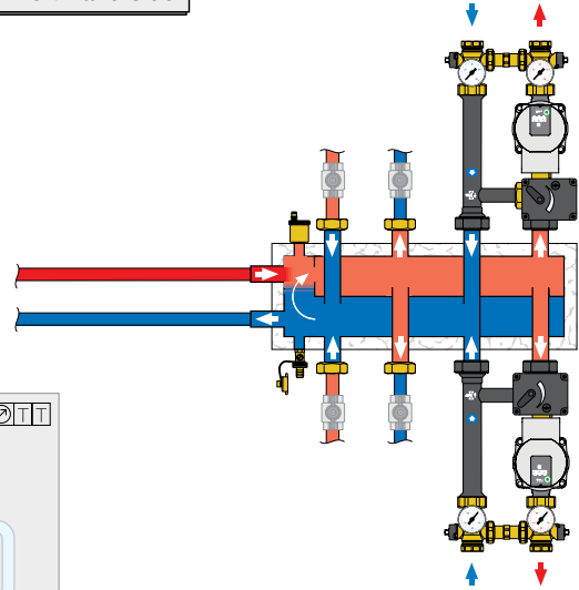
Configuration with SEPCOLL supplied from left-hand side
